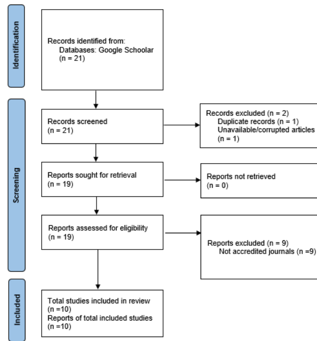
Figure 1. PRISMA Flowchart
