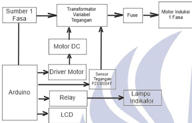
Gambar 10. Blok Diagram Prototype Penstabil Tegangan
