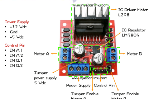
Gambar 6. Driver Motor tipe L298N ( Sumber : Widiarto, 2018 )
