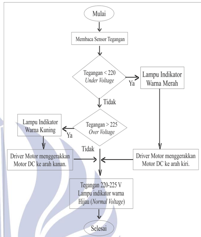
Gambar 12. Flow Chart Cara Kerja Prototype Penstabil Tegangan
