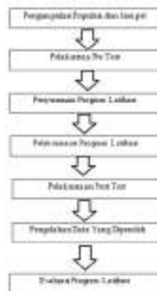
Gambar 1. Prosedur penelitian
