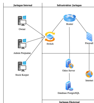
Figure 4 System Model Design
