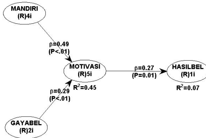
Gambar 2. Model Penelitian
