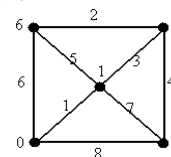
Gambar 1. Pelabelan Graceful
