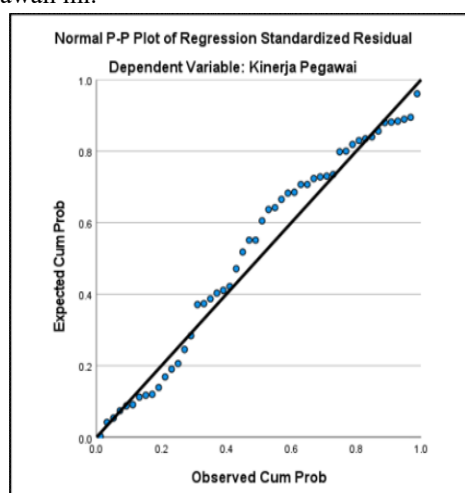
Gambar 1.2 Grafik Normal P-P Plot
